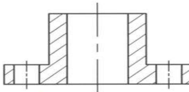
Front Sectional View
