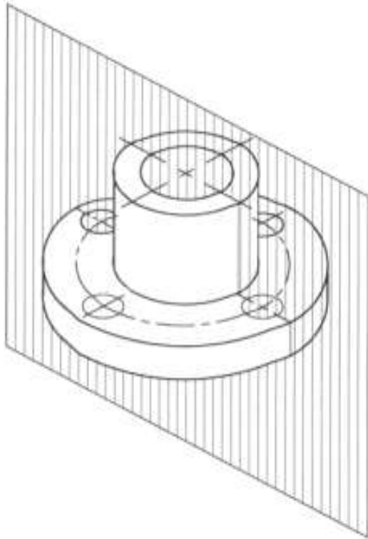
Figure 5.3.1: Object with Cutting Plane through Mid-Section
